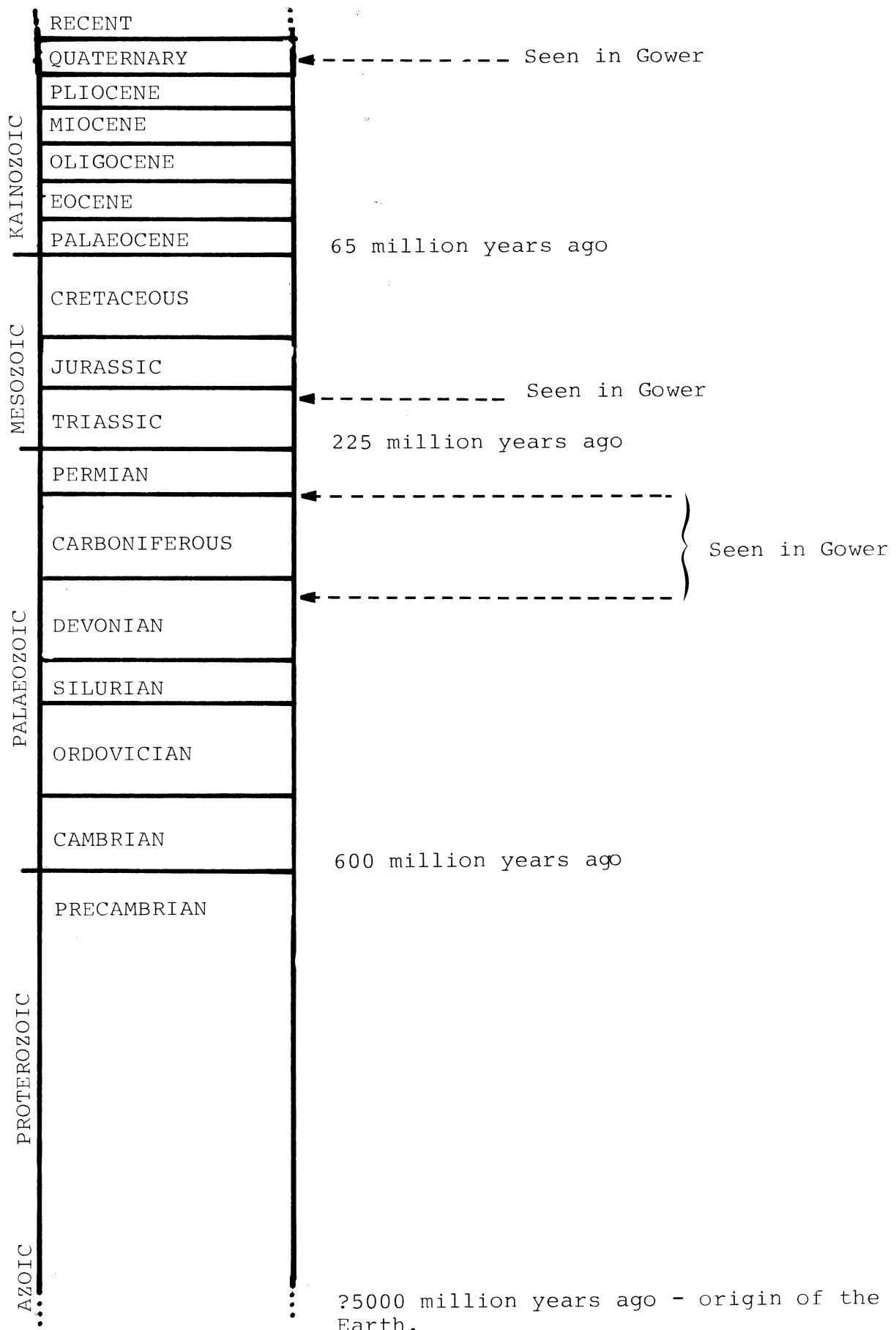
Fig.2 General Stratigraphic Table
