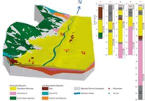
3D model of surficial geology of study site showing geomorphic features and hydrogeological heterogeneity at several depths
