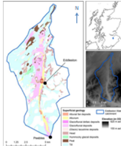
Location of study site in the Eddleston Water catchment showing superficial geology and sub-catchments
