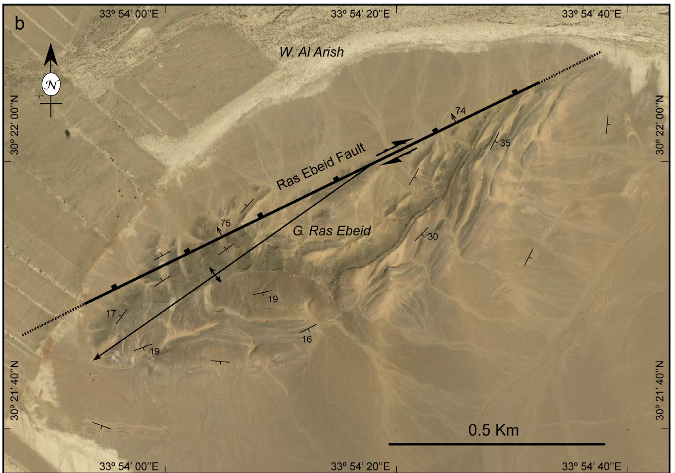
Fig. 2. (a) Google Earth image © 2013 DigitalGlobe of the Rishat Lehman Fault (RLF) and the southwestern part of the main Minsherah Fault (MMF). Lower Miocene basic igneous dike (d) is dextrally offset by the RLF for about 120 m. (b) Detailed Landsat TM image showing the structure of G. Ras Ebeid.
