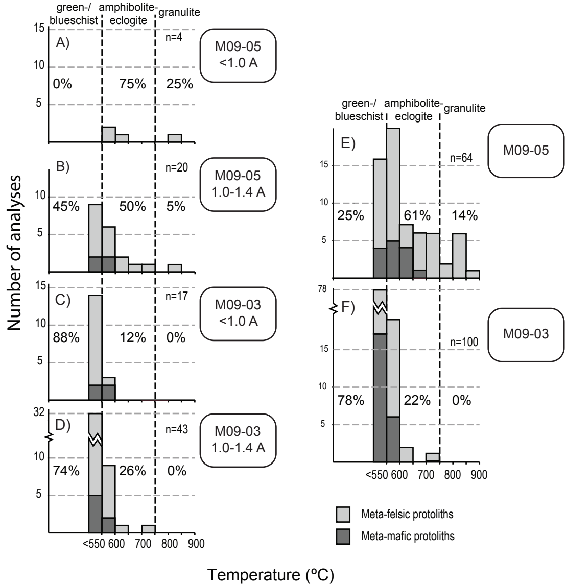
Appendix 2. A-D) Histograms of rutile temperature data from magnetic fractions. E, F) Magnetic and non-magnetic rutile data combined. Data from the magnetic fractions confirm the presence of high grade rutile in M09-05, and reproduce the dominantly greenschist to low amphibolite facies temperatures in M09-03 recorded in the non-magnetic fraction. The total proportion of meta-mafic rutile in the magnetic fractions are 17% (M09-05) and 18% (M09-03), slightly lower than in the non-magnetic fractions.
