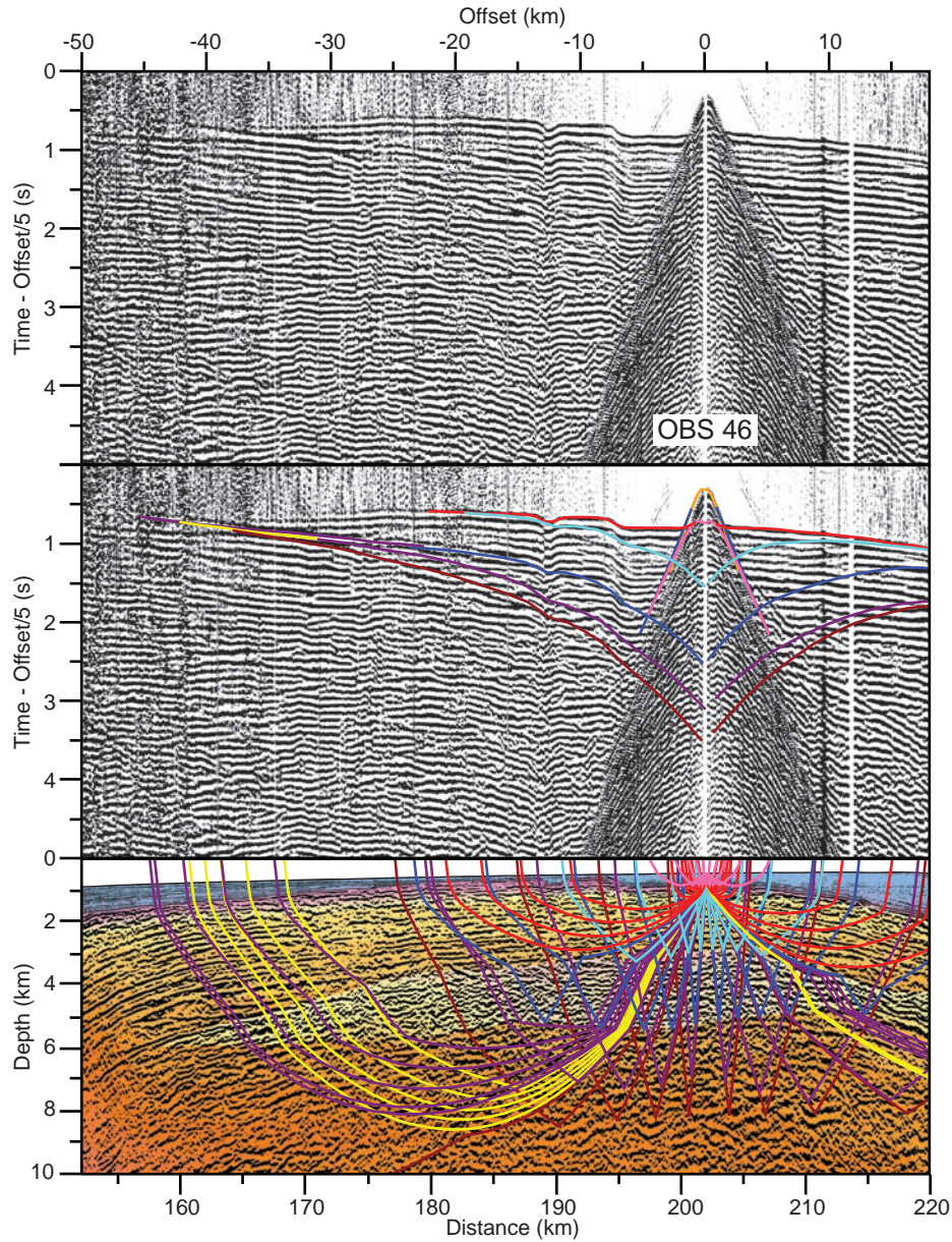
Fig S7. (Top) Record section for geophone data of OBS 46. A linear moveout at 5 km/s has been applied. Distances are measured from the north-northwestern end of the complete model (as in Roberts et al. 2009) and offsets are shot-receiver distances. (Middle) Record section with traveltime curves calculated by raytracing through the final velocity model and colour-coded by phases (see Figure 4 for legend). (Bottom) the corresponding ray path diagram with the same colour code as above. Only top basalt and deeper phases are shown for clarity. The seismic section was prestack depth migrated using the same final P-wave velocity model (colourmap) as is used in the raytracing. See text for modelling details. See Figure 8 in main paper for OBS location.
