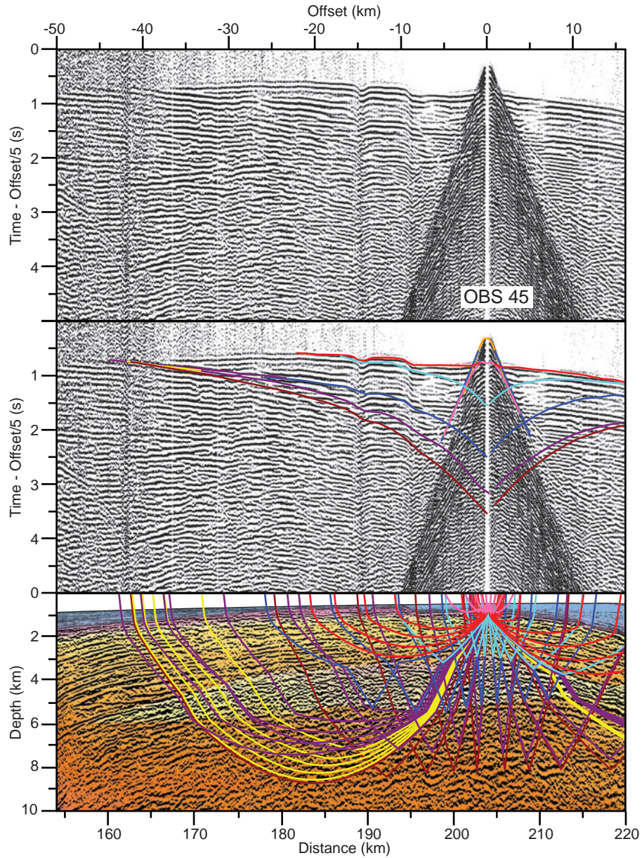
Fig S6. (Top) Record section for geophone data of OBS 45. A linear moveout at 5 km/s has been applied. Distances are measured from the north-northwestern end of the complete model (as in Roberts et al. 2009) and offsets are shot-receiver distances. (Middle) Record section with traveltime curves calculated by raytracing through the final velocity model and colour-coded by phases (see Figure 4 for legend). (Bottom) the corresponding ray path diagram with the same colour code as above. Only top basalt and deeper phases are shown for clarity. The seismic section was prestack depth migrated using the same final P-wave velocity model (colourmap) as is used in the raytracing. See text for modelling details. See Figure 8 in main paper for OBS location.
