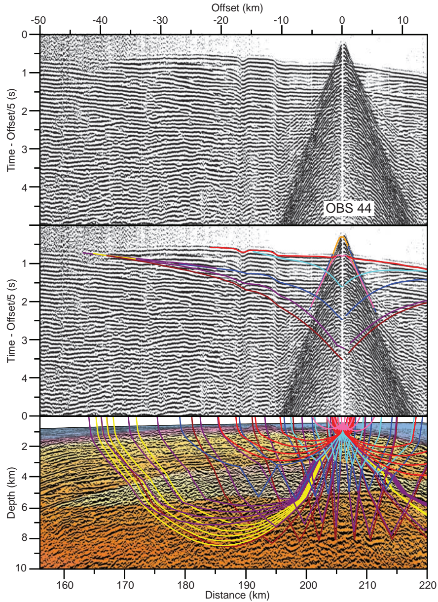
Fig S5. (Top) Record section for geophone data of OBS 44. A linear moveout at 5 km/s has been applied. Distances are measured from the north-northwestern end of the complete model (as in Roberts et al. 2009) and offsets are shot-receiver distances. (Middle) Record section with traveltime curves calculated by raytracing through the final velocity model and colour-coded by phases (see Figure 4 for legend). (Bottom) the corresponding ray path diagram with the same colour code as above. Only top basalt and deeper phases are shown for clarity. The seismic section was prestack depth migrated using the same final P-wave velocity model (colourmap) as is used in the raytracing. See text for modelling details. See Figure 8 in main paper for OBS location.
