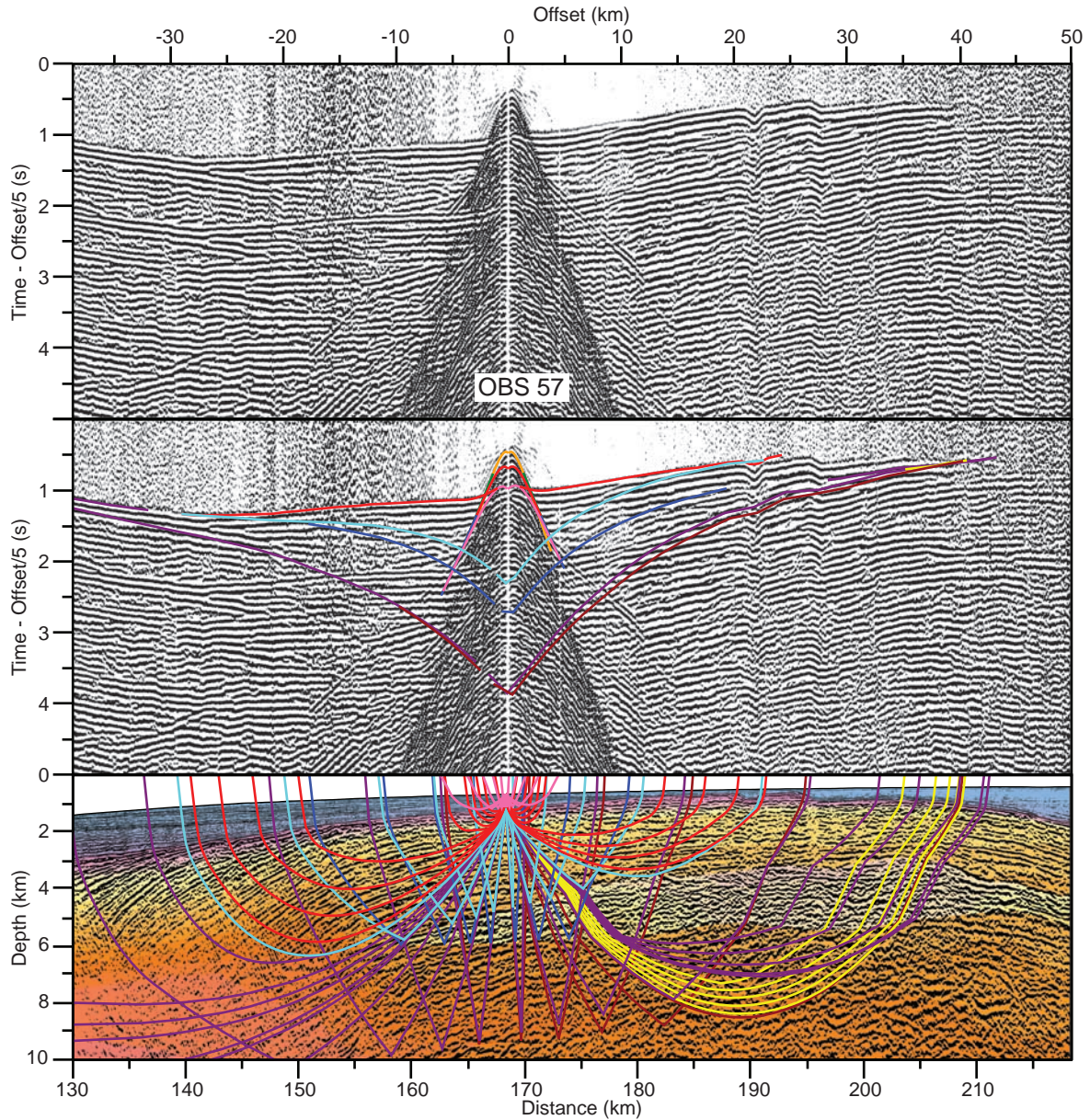
Fig S16. (Top) Record section for geophone data of OBS 57. A linear moveout at 5 km/s has been applied. Distances are measured from the north-northwestern end of the complete model (as in Roberts et al. 2009) and offsets are shot-receiver distances. (Middle) Record section with traveltime curves calculated by raytracing through the final velocity model and colour-coded by phases (see Figure 4 for legend). (Bottom) the corresponding ray path diagram with the same colour code as above. Only top basalt and deeper phases are shown for clarity. The seismic section was prestack depth migrated using the same final P-wave velocity model (colourmap) as is used in the raytracing. See text for modelling details. See Figure 8 in main paper for OBS location.
