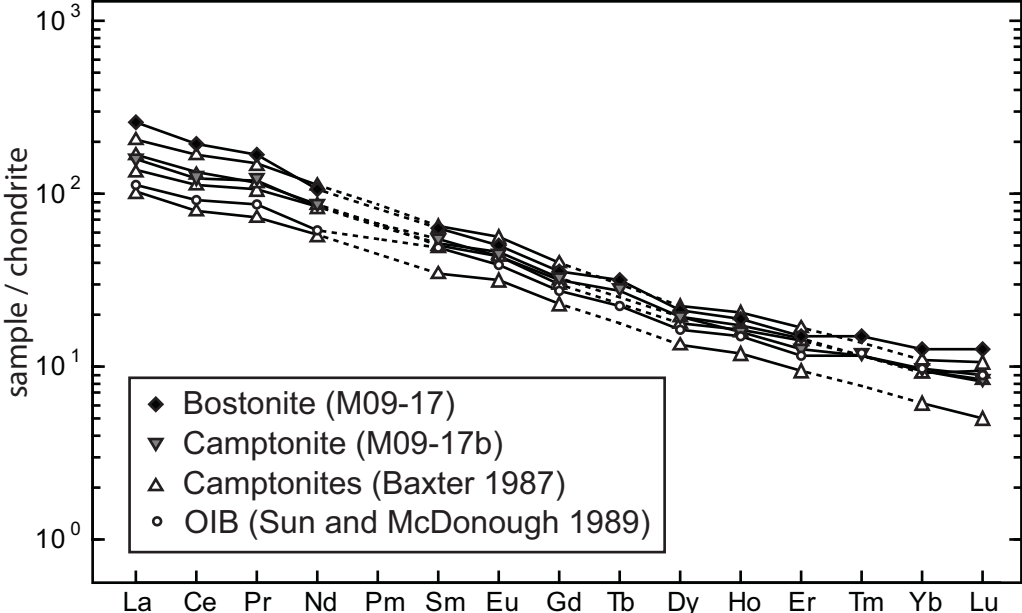
Appendix 5. REE diagram, chondrite normalized after Nakamura (1974).
