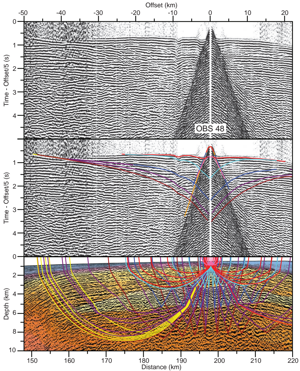
Fig S9. (Top) Record section for geophone data of OBS 48. A linear moveout at 5 km/s has been applied. Distances are measured from the north-northwestern end of the complete model (as in Roberts et al. 2009) and offsets are shot-receiver distances. (Middle) Record section with traveltime curves calculated by raytracing through the final velocity model and colour-coded by phases (see Figure 4 for legend). (Bottom) the corresponding ray path diagram with the same colour code as above. Only top basalt and deeper phases are shown for clarity. The seismic section was prestack depth migrated using the same final P-wave velocity model (colourmap) as is used in the raytracing. See text for modelling details. See Figure 8 in main paper for OBS location.
