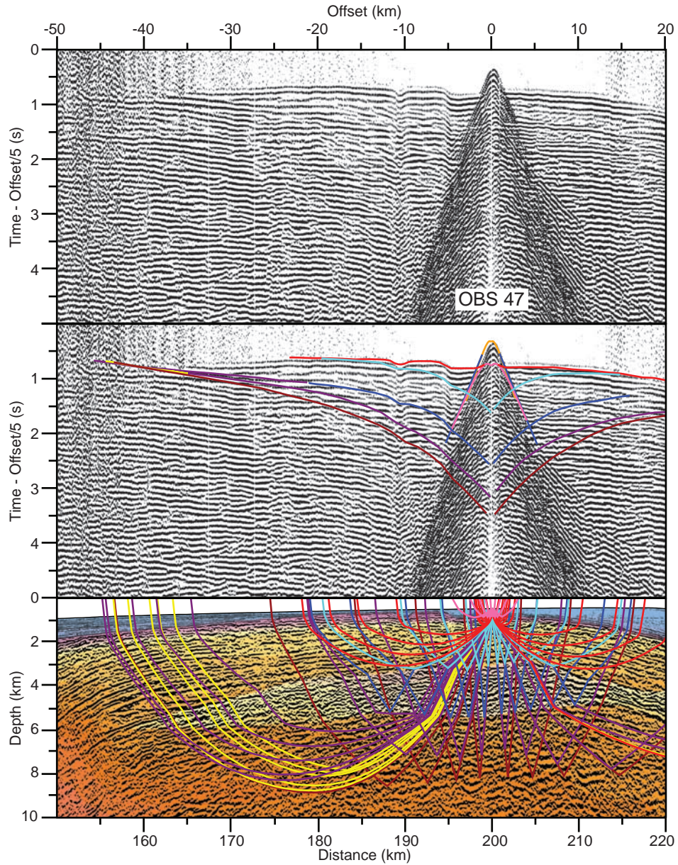
Fig S8. (Top) Record section for geophone data of OBS 47. A linear moveout at 5 km/s has been applied. Distances are measured from the north-northwestern end of the complete model (as in Roberts et al. 2009) and offsets are shot-receiver distances. (Middle) Record section with traveltime curves calculated by raytracing through the final velocity model and colour-coded by phases (see Figure 4 for legend). (Bottom) the corresponding ray path diagram with the same colour code as above. Only top basalt and deeper phases are shown for clarity. The seismic section was prestack depth migrated using the same final P-wave velocity model (colourmap) as is used in the raytracing. See text for modelling details. See Figure 8 in main paper for OBS location.
