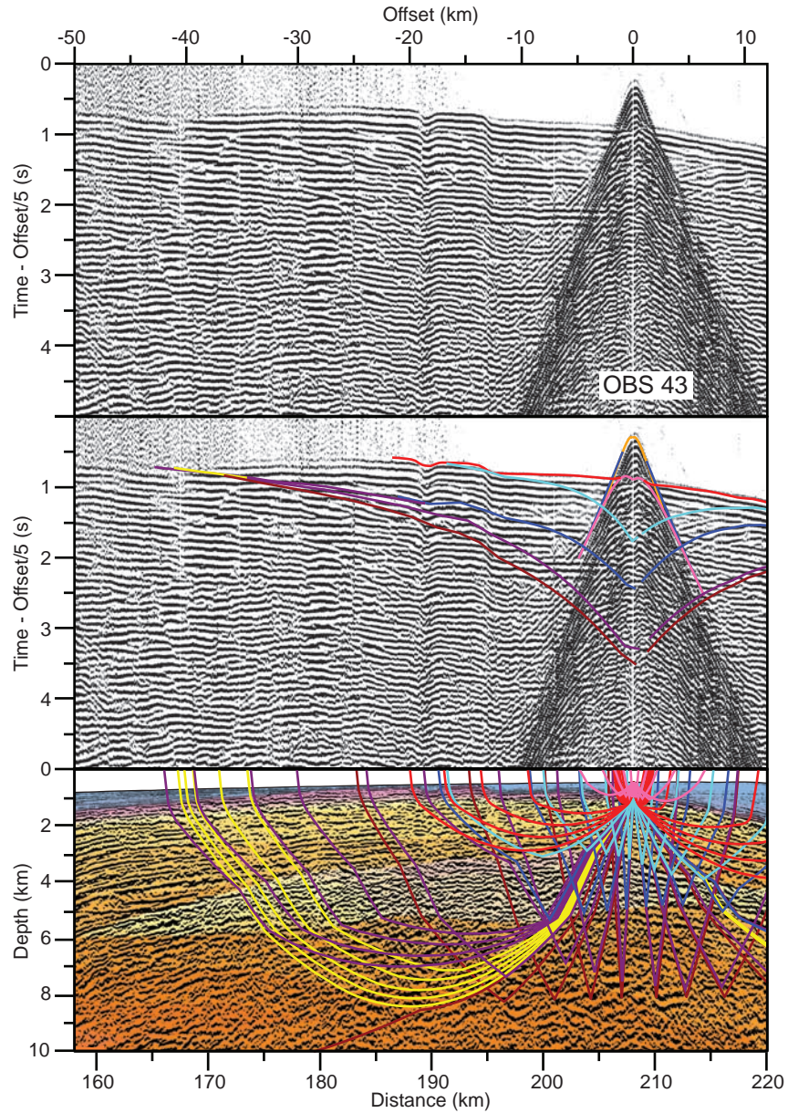
Fig S4. (Top) Record section for geophone data of OBS 43. A linear moveout at 5 km/s has been applied. Distances are measured from the north-northwestern end of the complete model (as in Roberts et al. 2009) and offsets are shot-receiver distances. (Middle) Record section with traveltime curves calculated by raytracing through the final velocity model and colour-coded by phases (see Figure 4 for legend). (Bottom) the corresponding ray path diagram with the same colour code as above. Only top basalt and deeper phases are shown for clarity. The seismic section was prestack depth migrated using the same final P-wave velocity model (colourmap) as is used in the raytracing. See text for modelling details. See Figure 8 in main paper for OBS location.
