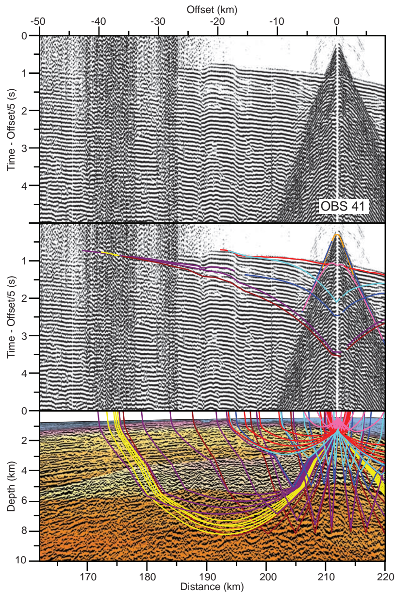
Fig S2. (Top) Record section for geophone data of OBS 41. A linear moveout at 5 km/s has been applied. Distances are measured from the north-northwestern end of the complete model (as in Roberts et al. 2009) and offsets are shot-receiver distances. (Middle) Record section with traveltime curves calculated by raytracing through the final velocity model and colour-coded by phases (see Figure 4 for legend). (Bottom) the corresponding ray path diagram with the same colour code as above. Only top basalt and deeper phases are shown for clarity. The seismic section was prestack depth migrated using the same final P-wave velocity model (colourmap) as is used in the raytracing. See text for modelling details. See Figure 8 in main paper for OBS location.
