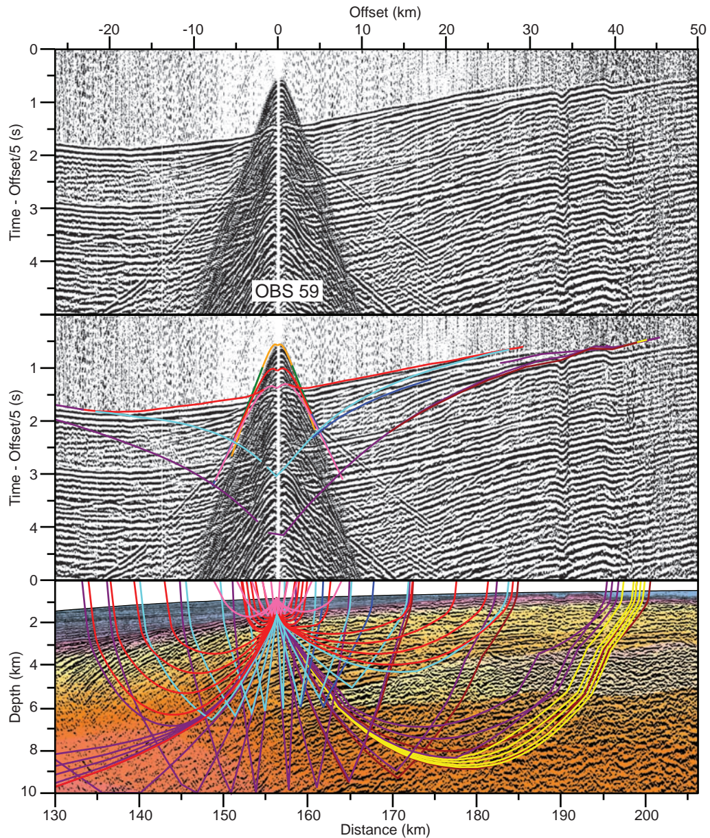
Fig S17. (Top) Record section for geophone data of OBS 59. A linear moveout at 5 km/s has been applied. Distances are measured from the north-northwestern end of the complete model (as in Roberts et al. 2009) and offsets are shot-receiver distances. (Middle) Record section with traveltime curves calculated by raytracing through the final velocity model and colour-coded by phases (see Figure 4 for legend). (Bottom) the corresponding ray path diagram with the same colour code as above. Only top basalt and deeper phases are shown for clarity. The seismic section was prestack depth migrated using the same final P-wave velocity model (colourmap) as is used in the raytracing. See text for modelling details. See Figure 8 in main paper for OBS location.
