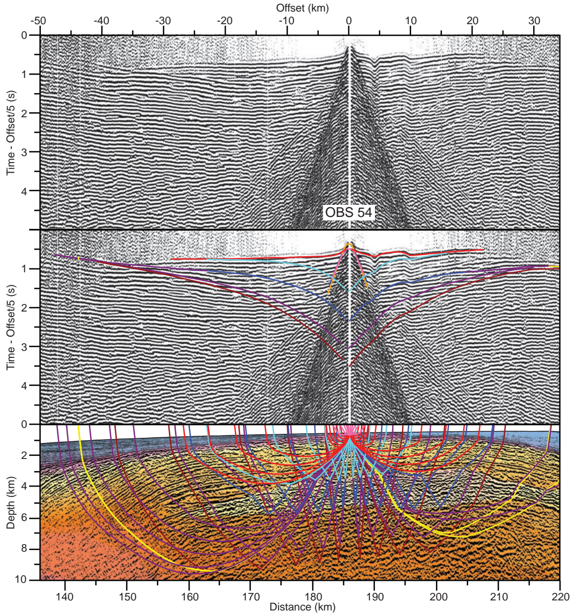
Fig S13. (Top) Record section for geophone data of OBS 54. A linear moveout at 5 km/s has been applied. Distances are measured from the north-northwestern end of the complete model (as in Roberts et al. 2009) and offsets are shot-receiver distances. (Middle) Record section with traveltime curves calculated by raytracing through the final velocity model and colour-coded by phases (see Figure 4 for legend). (Bottom) the corresponding ray path diagram with the same colour code as above. Only top basalt and deeper phases are shown for clarity. The seismic section was prestack depth migrated using the same final P-wave velocity model (colourmap) as is used in the raytracing. See text for modelling details. See Figure 8 in main paper for OBS location.
