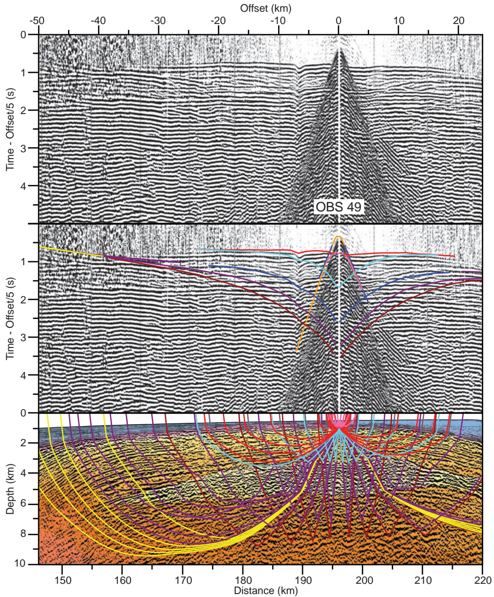
Fig S10. (Top) Record section for geophone data of OBS 49. A linear moveout at 5 km/s has been applied. Distances are measured from the north-northwestern end of the complete model (as in Roberts et al. 2009) and offsets are shot-receiver distances. (Middle) Record section with traveltime curves calculated by raytracing through the final velocity model and colour-coded by phases (see Figure 4 for legend). (Bottom) the corresponding ray path diagram with the same colour code as above. Only top basalt and deeper phases are shown for clarity. The seismic section was prestack depth migrated using the same final P-wave velocity model (colourmap) as is used in the raytracing. See text for modelling details. See Figure 8 in main paper for OBS location.
