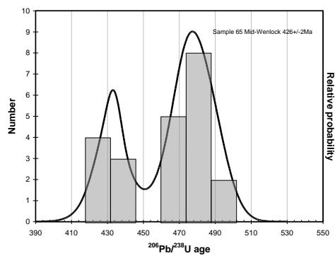
PDP of young (<500Ma) grains in N5065
