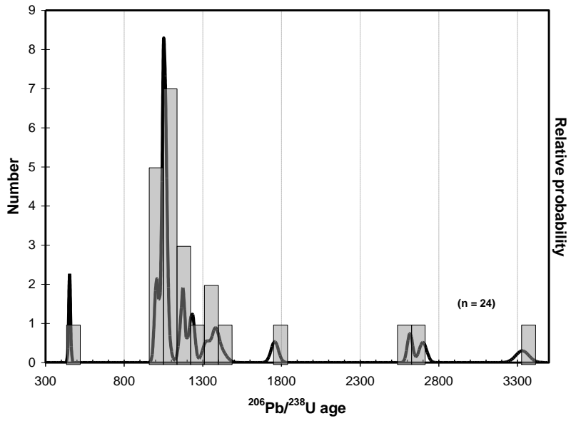
Age distribution plots for Sample N5068
