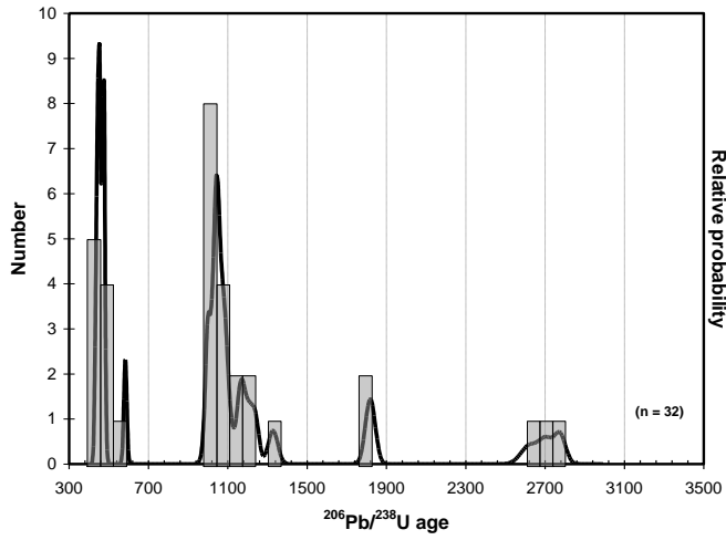
Age distribution for sample N5067
