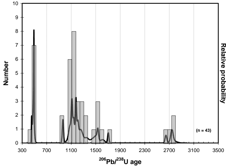
Age distribution plots for Sample N5071
