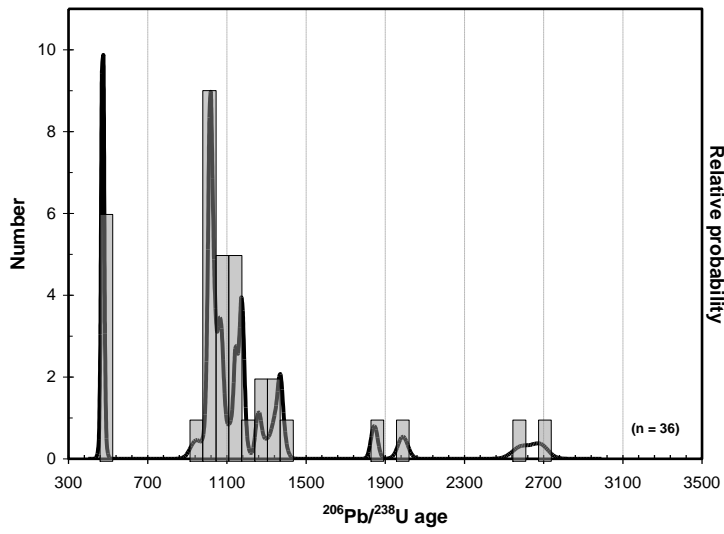
Age distribution plots for Sample N5075
