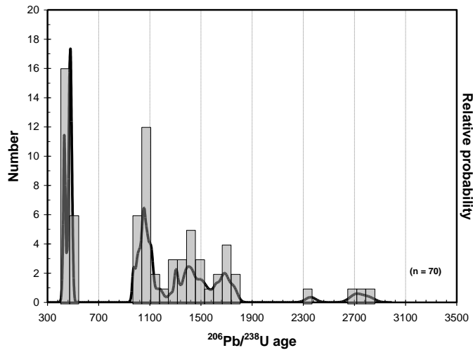
Probability density plot for sample N5065
