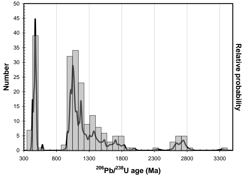
Combined Probability density plot
