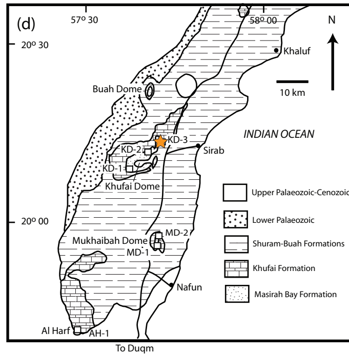
Figure S1: Outcrop map of Oman (a) and geological maps showing the sampled localities (stars) for detrital zircons of the Mirbat Group (b), the Abu Mahara Group in the Jabal Akhdar (Ghubrah in green; Saqlah in red; Fiq in black) (c), and the Masirah Bay Formation of the Huqf area (d). Map(c) adapted from Leather et al. (2001) and (d) adapted from Allen & Leather (2006).
