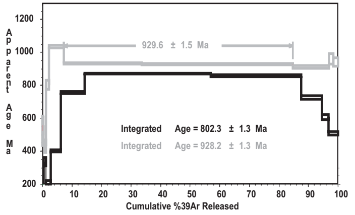
Figure 1r. Dibuya Gneiss, Hornblende A-59
