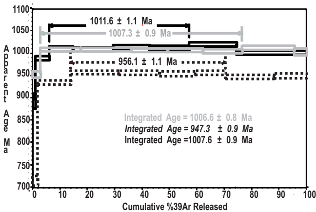
Figure 1g. Margaritas Gneiss, Biotite C-302
