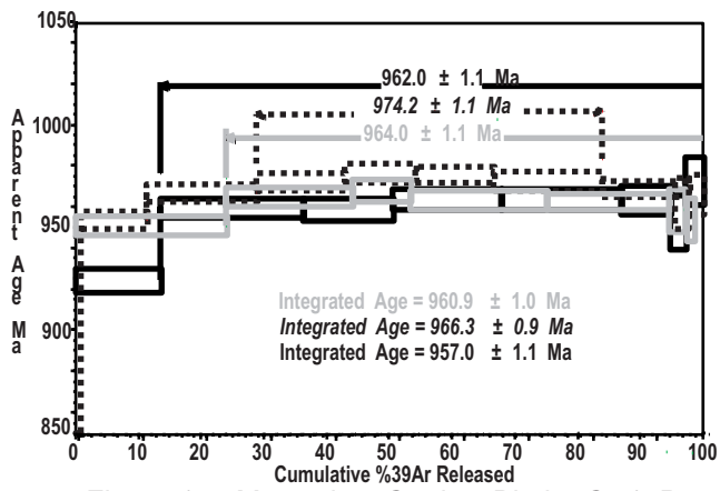
Figure 1m. Margaritas Gneiss, Biotite Gr-15P
