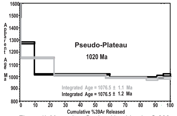
Figure 1j. Margaritas Gneiss, Hornblende C-299
