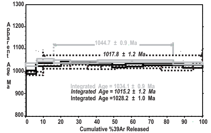
Figure 1h. Margaritas Gneiss, Biotite C-271
