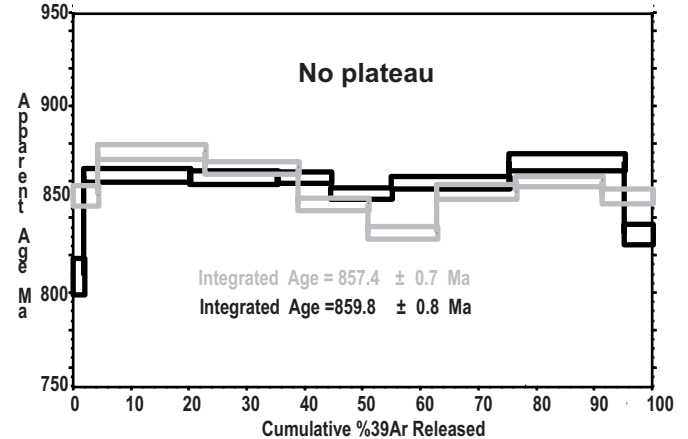
Figure 1d. Vergel Granulite, biotite D-982
