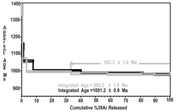
Figure 1l. Margaritas Gneiss, Hornblende C-32
