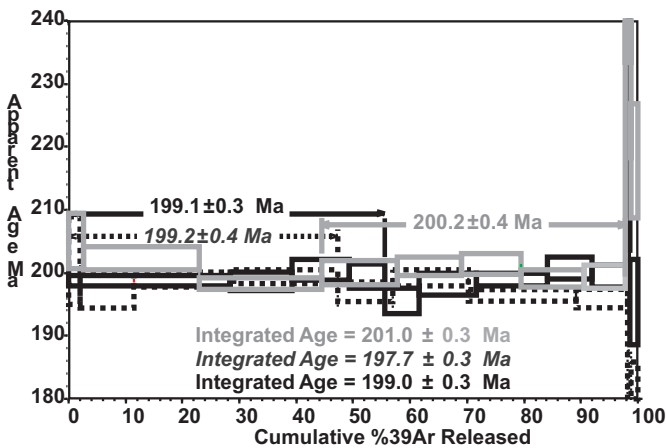
Figure 1w. Bucaramanga Gneiss, Biotite PCM-1105
