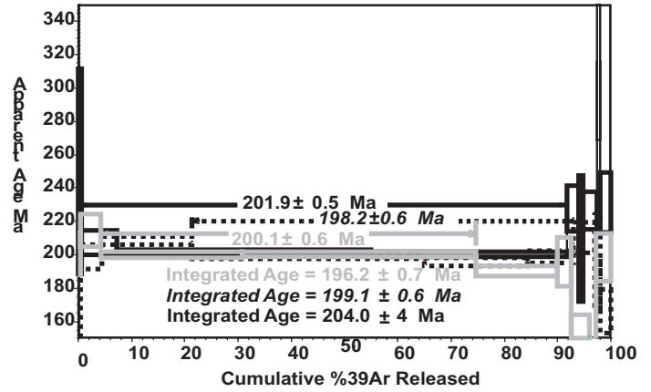
Figure 1t. Bucaramanga Gneiss, Hornblende PCM-815
