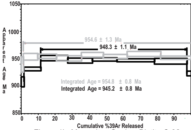
Figure 1k. Margaritas Gneiss, Biotite C-32
