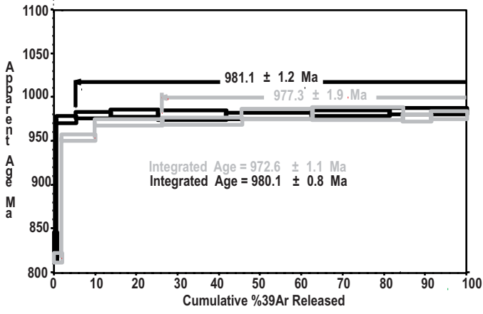
Figure 1i. Margaritas Gneiss, Biotite C-299
