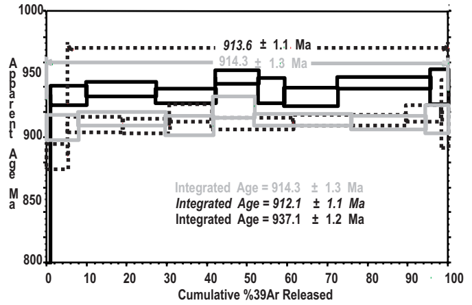
Figure 1b. Vergel Granulite, biotite GR-29
