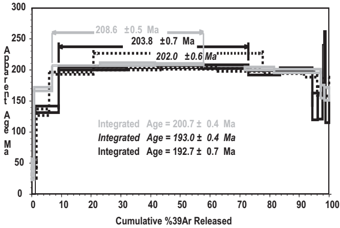
Figure 1s. Bucaramanga Gneiss, Biotite PCM-815
