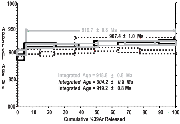
Figure 1a. Vergel Granulite, Biotite V-332
