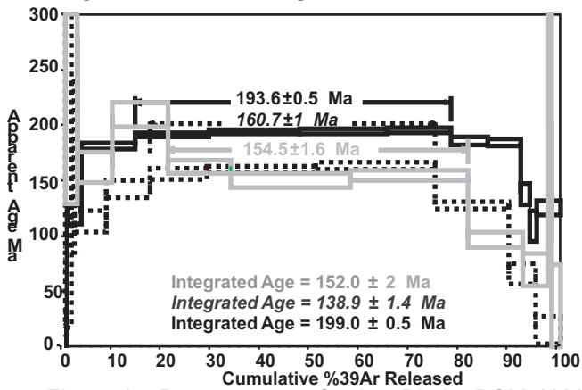
Figure 1u. Bucaramanga Gneiss, Biotite PCM-1102
