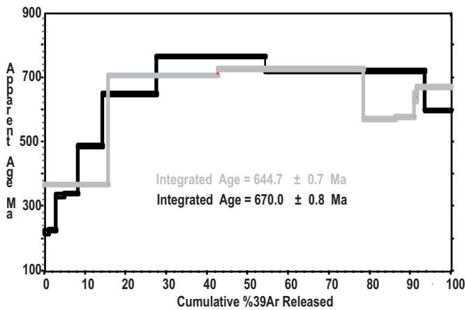
Figure 1o. Guapoton-Mancagua Gneiss, Hornblende V-198
