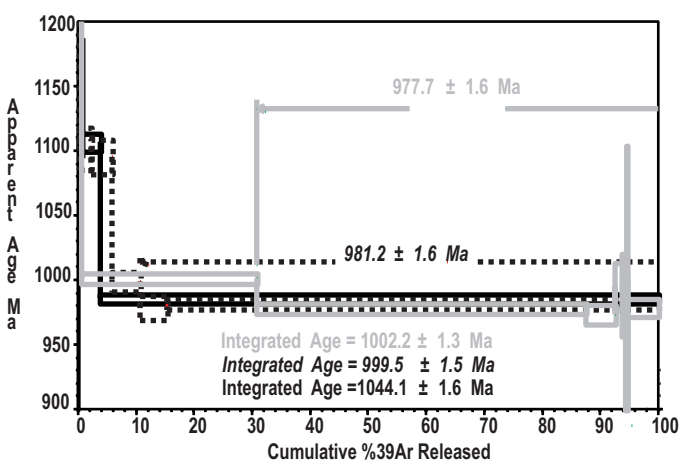
Figure 1f. Vergel Granulite, Hornblende V-309
