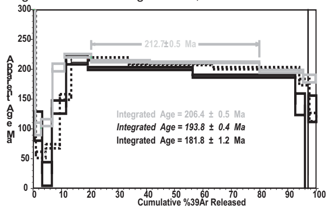
Figure 1v. Bucaramanga Gneiss, Hornblende PCM-1102
