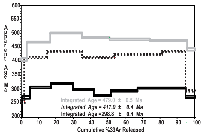
Figure 1n. Guapoton-Mancagua Gneiss, Biotite V-198
