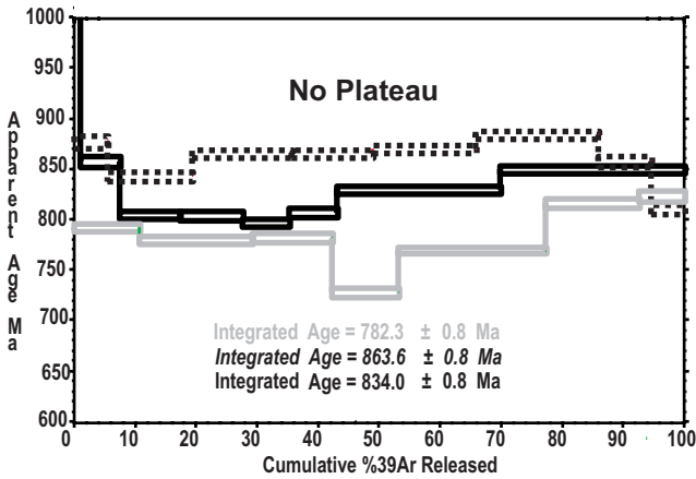
Figure 1c. Vergel Granulite, Biotite D-986
