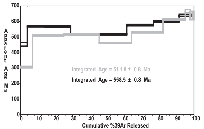
Figure 1p. Dibuya Gneiss, Biotite A-49
