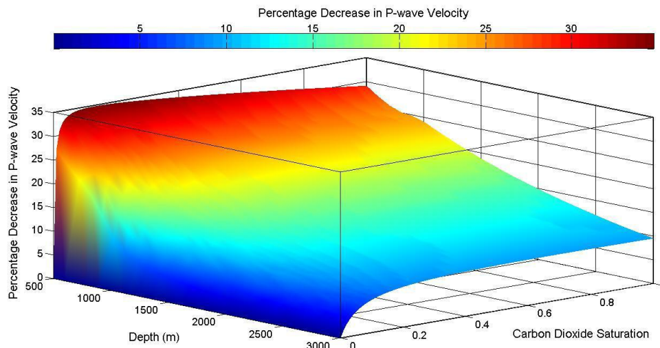
Figure 1 Percentage decrease in P-wave velocity ( V_p ) resulting from the injection of different saturations of CO 2 into sandstone reservoirs found between 500 and 3000m depth. The significant drop in V_p caused by small CO 2 saturations indicate that CO 2 location could be detected at all depths. In addition inferring saturation from V_p may be possible for saturations up to 40%, but higher saturations appear to be indistinguishable.
