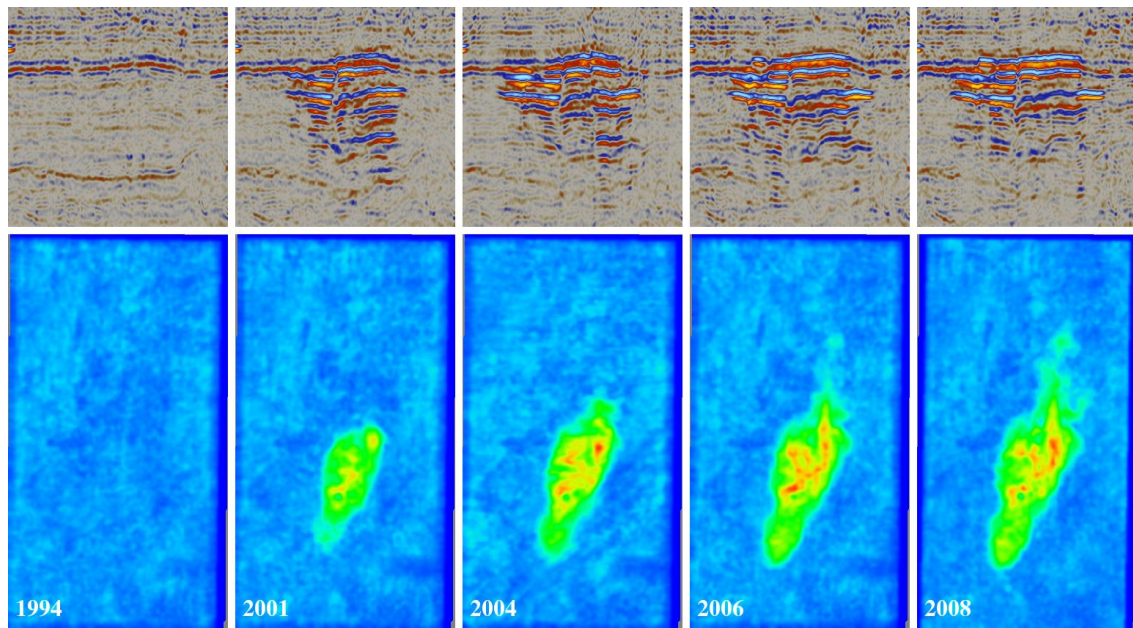
Figure 1. Time lapse response of a growing CO 2 plume at Sleipner, North Sea.
